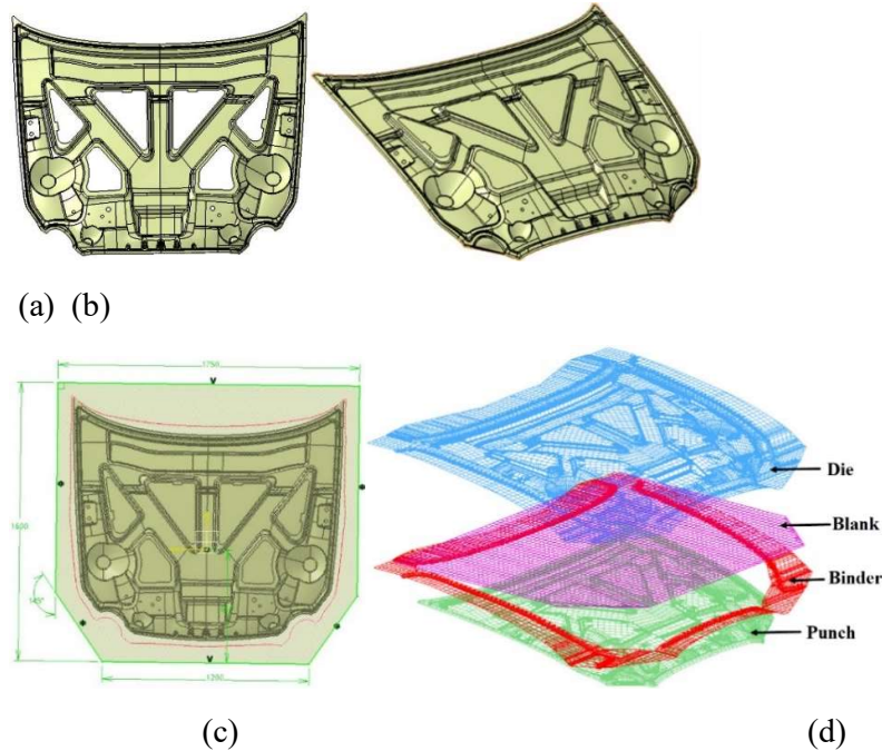
Fig. 1. The hood inner panel for study stamping process: (a) Finished model; (b) 3D stamping model; (c) Blank size; (d) FEM model for simulation
